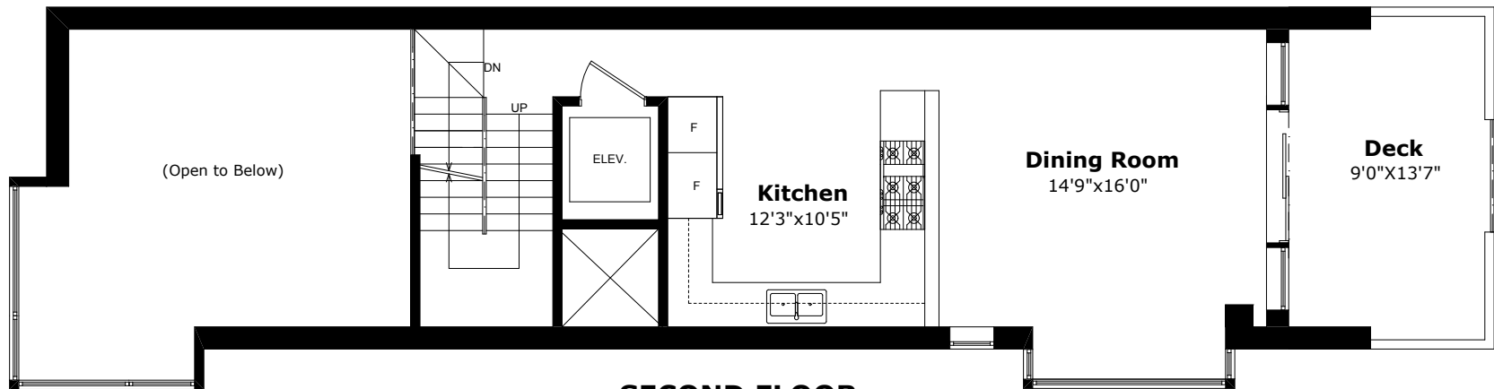
SECOND FLOOR
